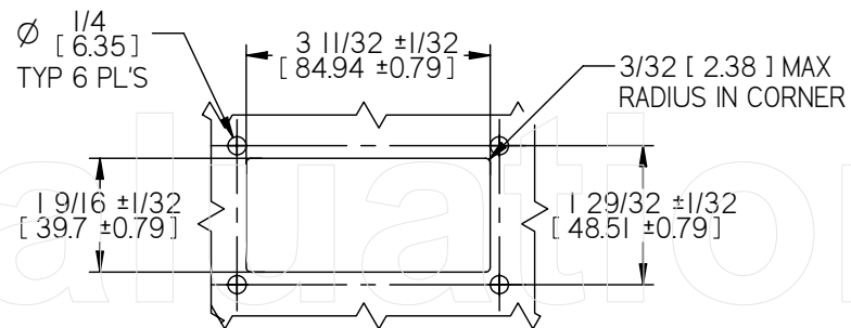
PANEL CUTOUT
